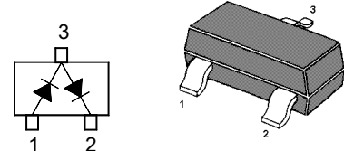
Marking Code: PX SOT-23 Plastic Package
